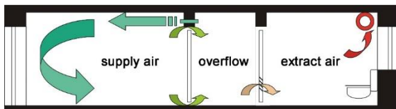
Zoning of the comfort ventilation systems with supply and extract air and heat recovery
